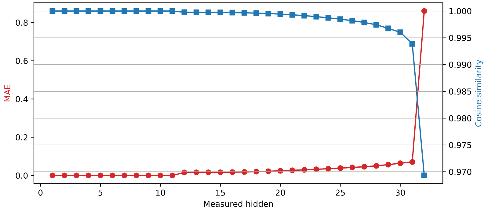
Mistral-7B-Instruct-v0.3 | Quantized layer 11 | float16 → int4
