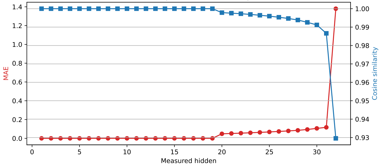
Mistral-7B-Instruct-v0.3 | Quantized layer 19 | float16 \rightarrow int4
