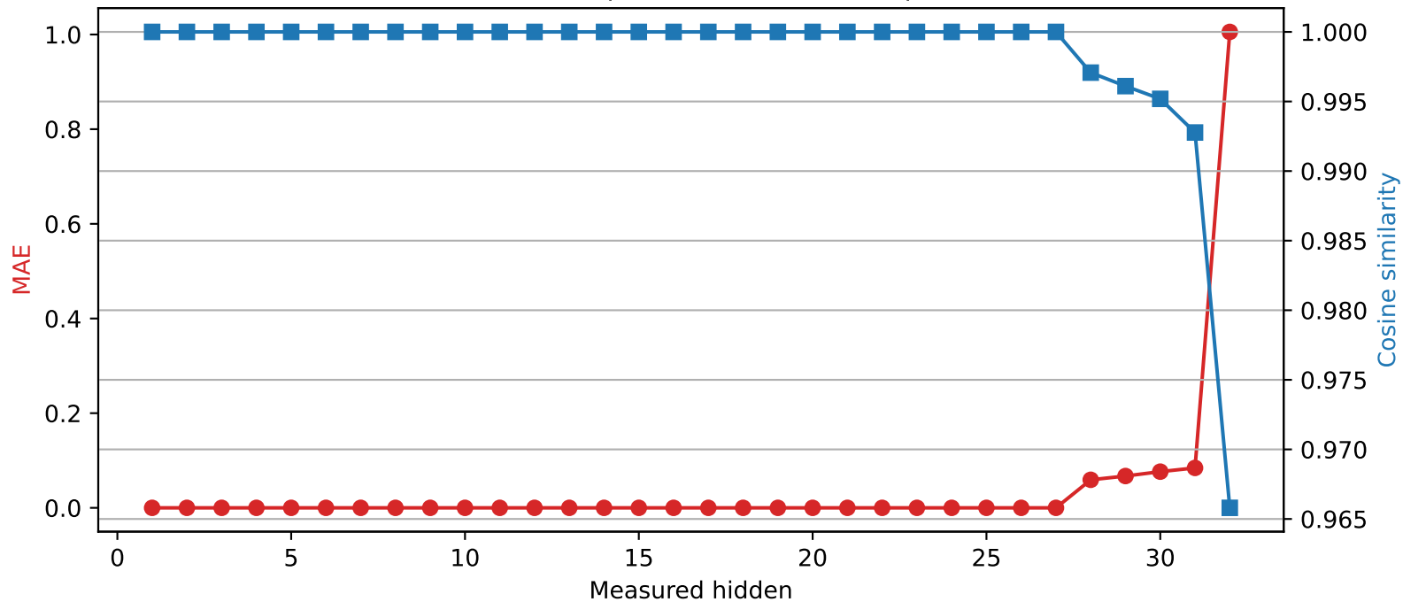
Mistral-7B-Instruct-v0.3 | Quantized layer 27 | float16 → int4
