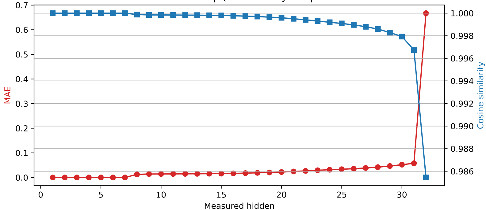
Mistral-7B-Instruct-v0.3 | Quantized layer 7 | float16 \rightarrow int4
