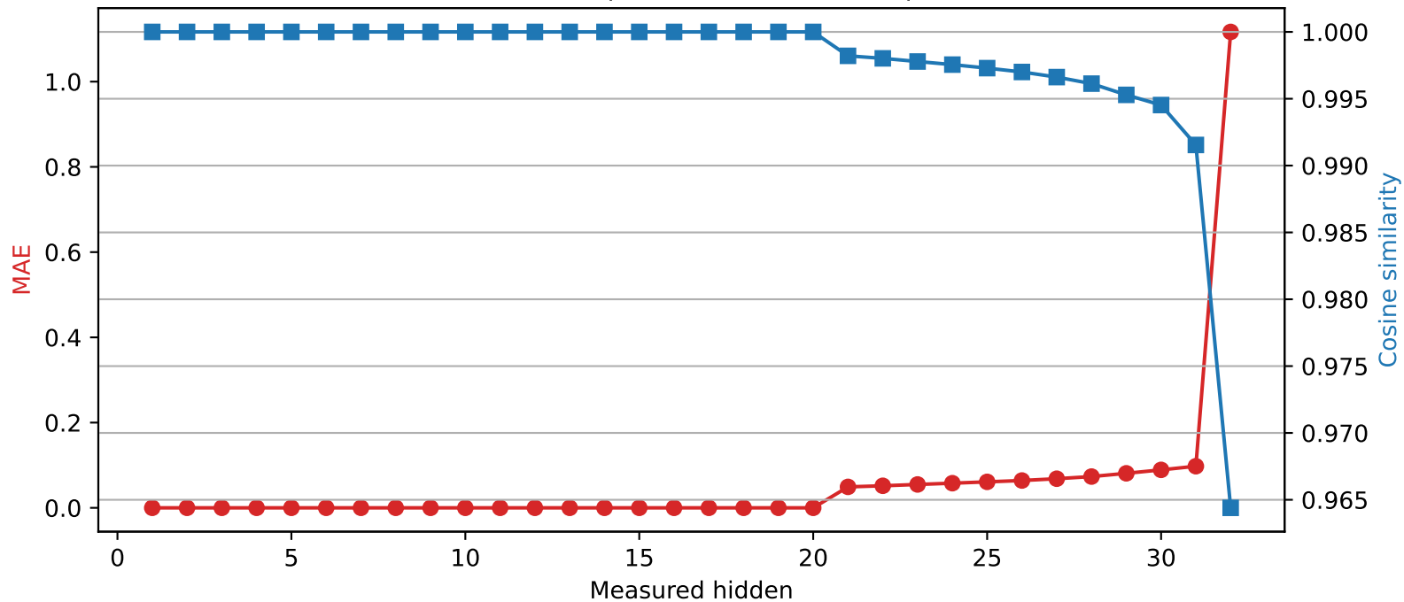
Mistral-7B-Instruct-v0.3 | Quantized layer 20 | float16 → int4
