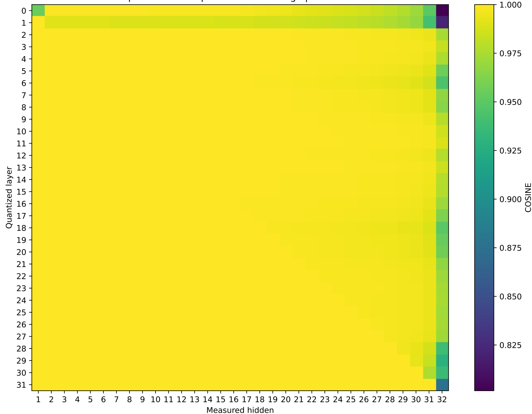
Mistral-7B-Instruct-v0.3 Prompt 3: cos sim representation damage | float16 \rightarrow int4
