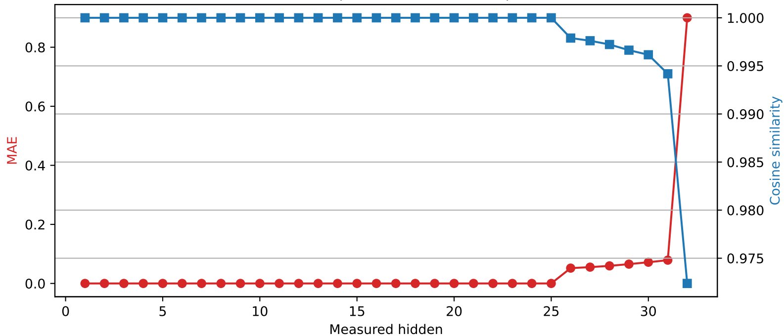
Mistral-7B-Instruct-v0.3 | Quantized layer 25 | float16 → int4
