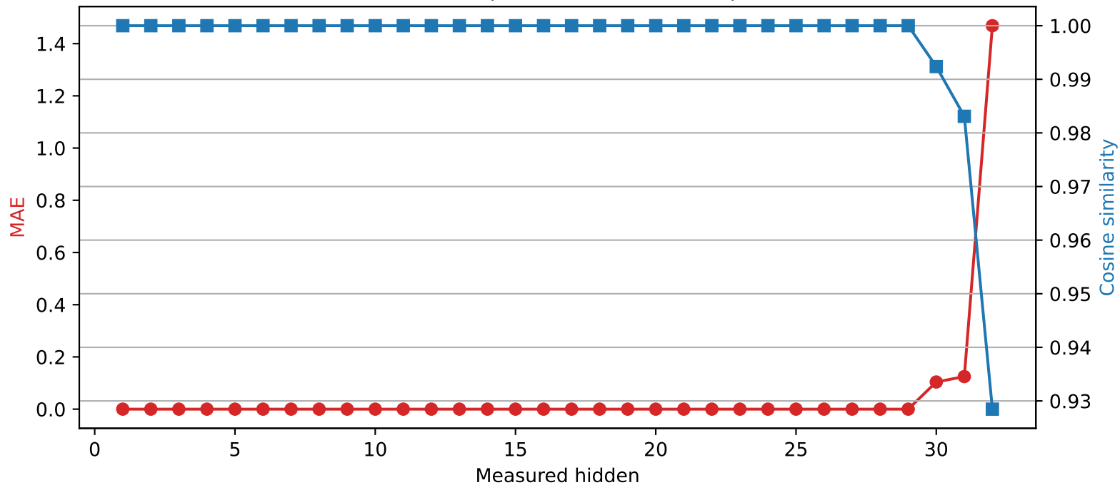
Mistral-7B-Instruct-v0.3 | Quantized layer 29 | float16 → int4
