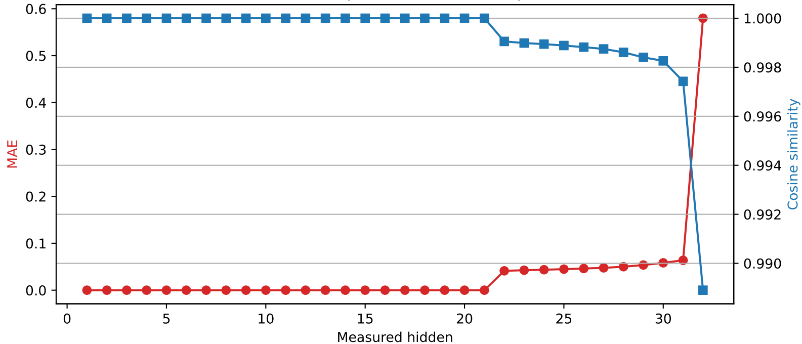
Mistral-7B-Instruct-v0.3 | Quantized layer 21 | float16 \rightarrow int4
