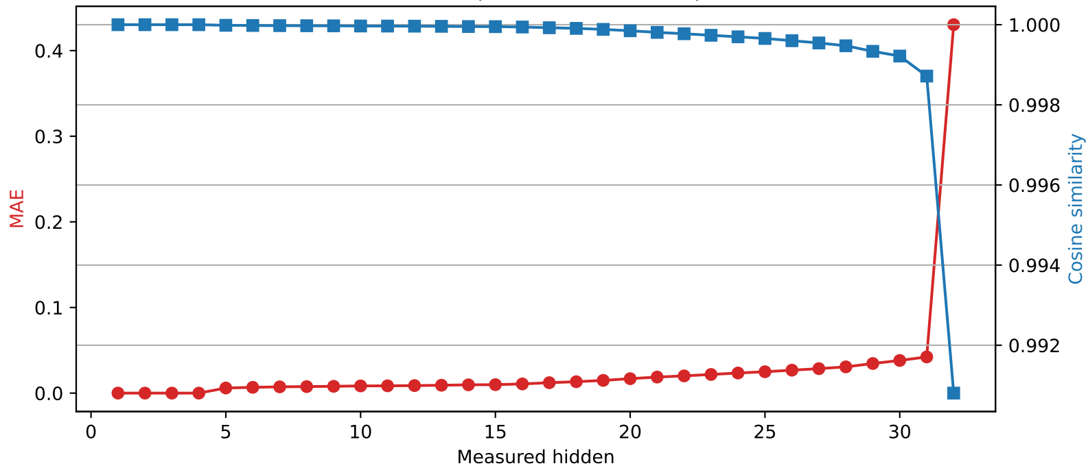
Mistral-7B-Instruct-v0.3 | Quantized layer 4 | float32 → int4
