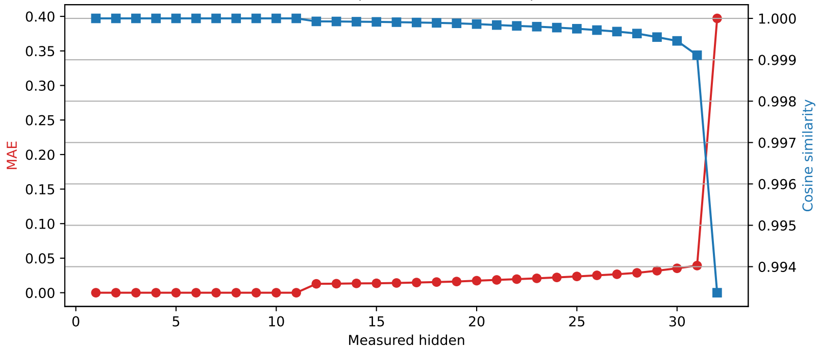
Mistral-7B-Instruct-v0.3 | Quantized layer 11 | float32 \rightarrow int4
