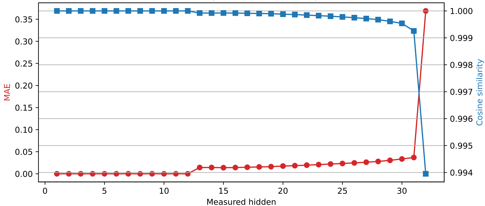
Mistral-7B-Instruct-v0.3 | Quantized layer 12 | float32 → int4
