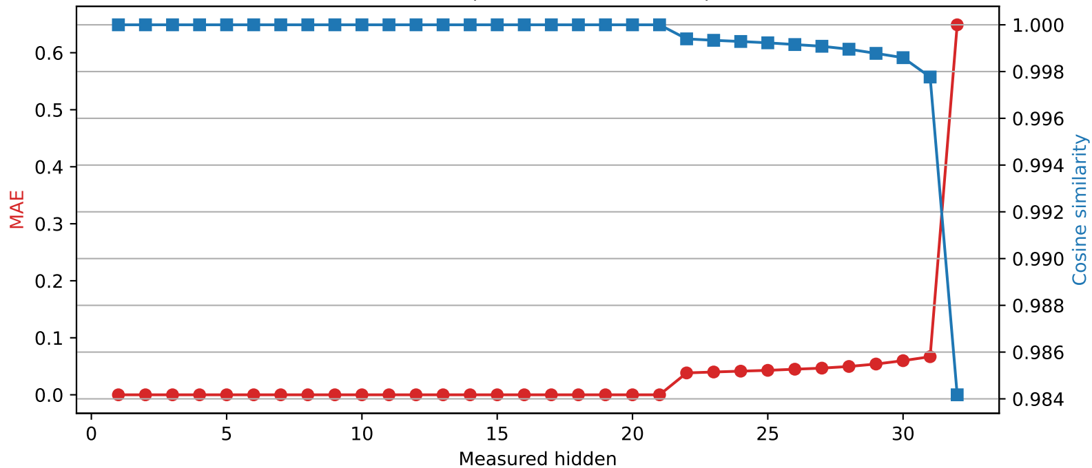
Mistral-7B-Instruct-v0.3 | Quantized layer 21 | float32 → int4
