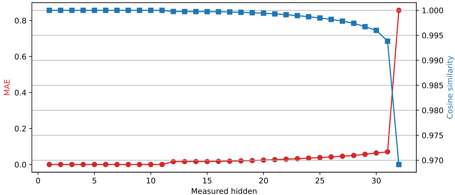
Mistral-7B-Instruct-v0.3 | Quantized layer 11 | float32 → int4
