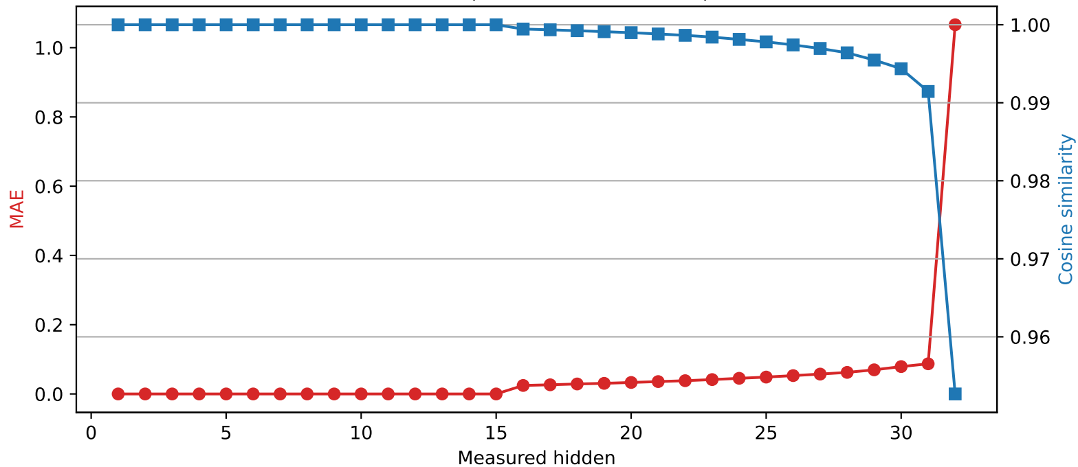
Mistral-7B-Instruct-v0.3 | Quantized layer 15 | float32 → int4
