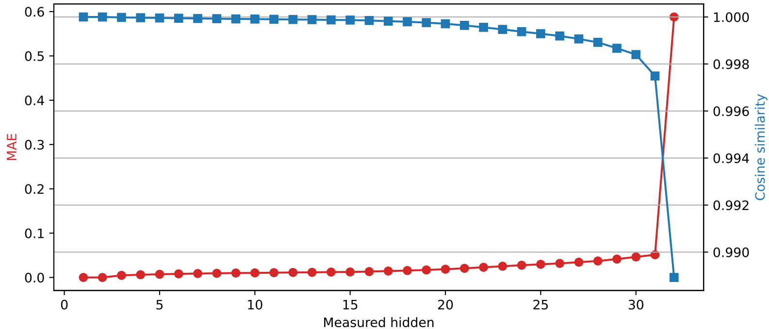
Mistral-7B-Instruct-v0.3 | Quantized layer 2 | float32 → int4
