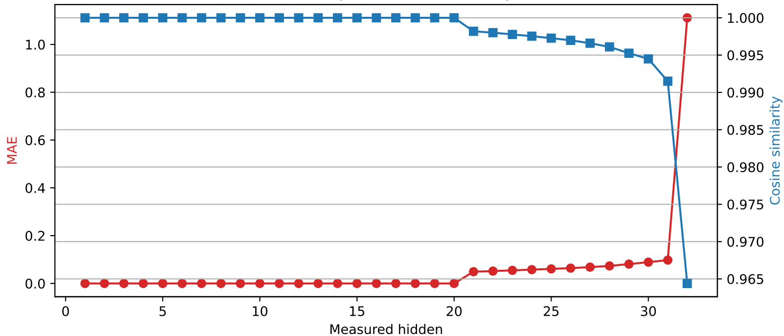
Mistral-7B-Instruct-v0.3 | Quantized layer 20 | float32 \rightarrow int4
