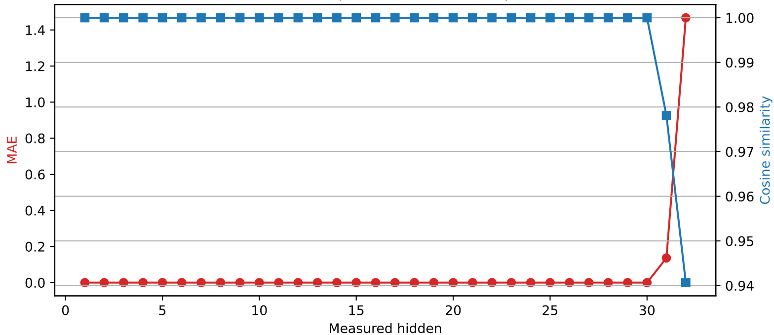
Mistral-7B-Instruct-v0.3 | Quantized layer 30 | float32 → int4
