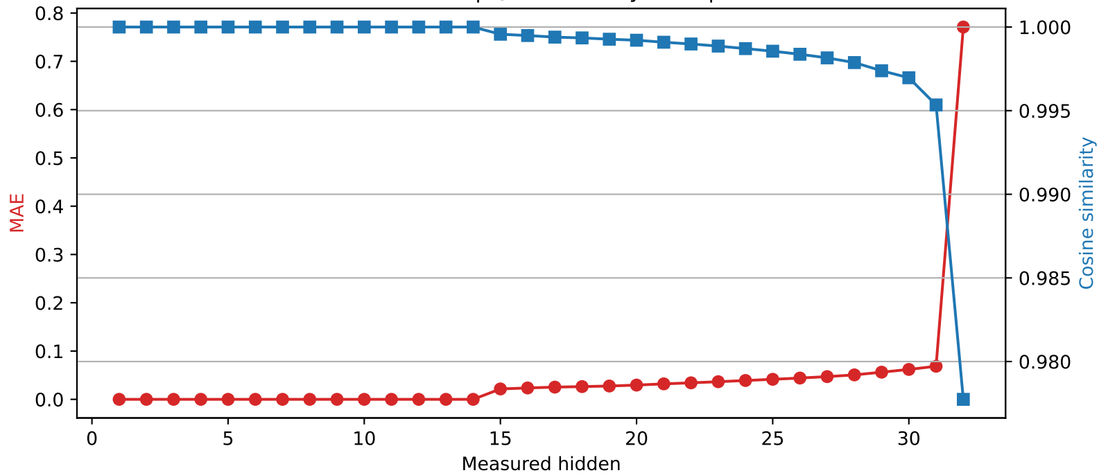
Mistral-7B-Instruct-v0.3 | Quantized layer 14 | float32 → int4
