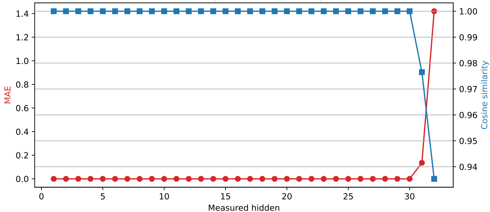
Mistral-7B-Instruct-v0.3 | Quantized layer 30 | float32 \rightarrow int4
