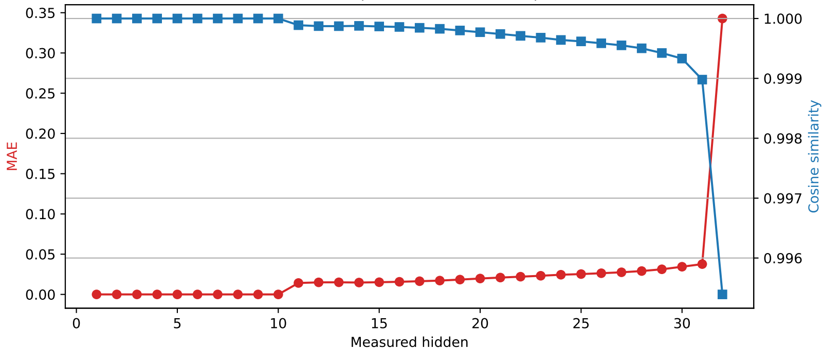
Mistral-7B-Instruct-v0.3 | Quantized layer 10 | float32 \rightarrow int4
