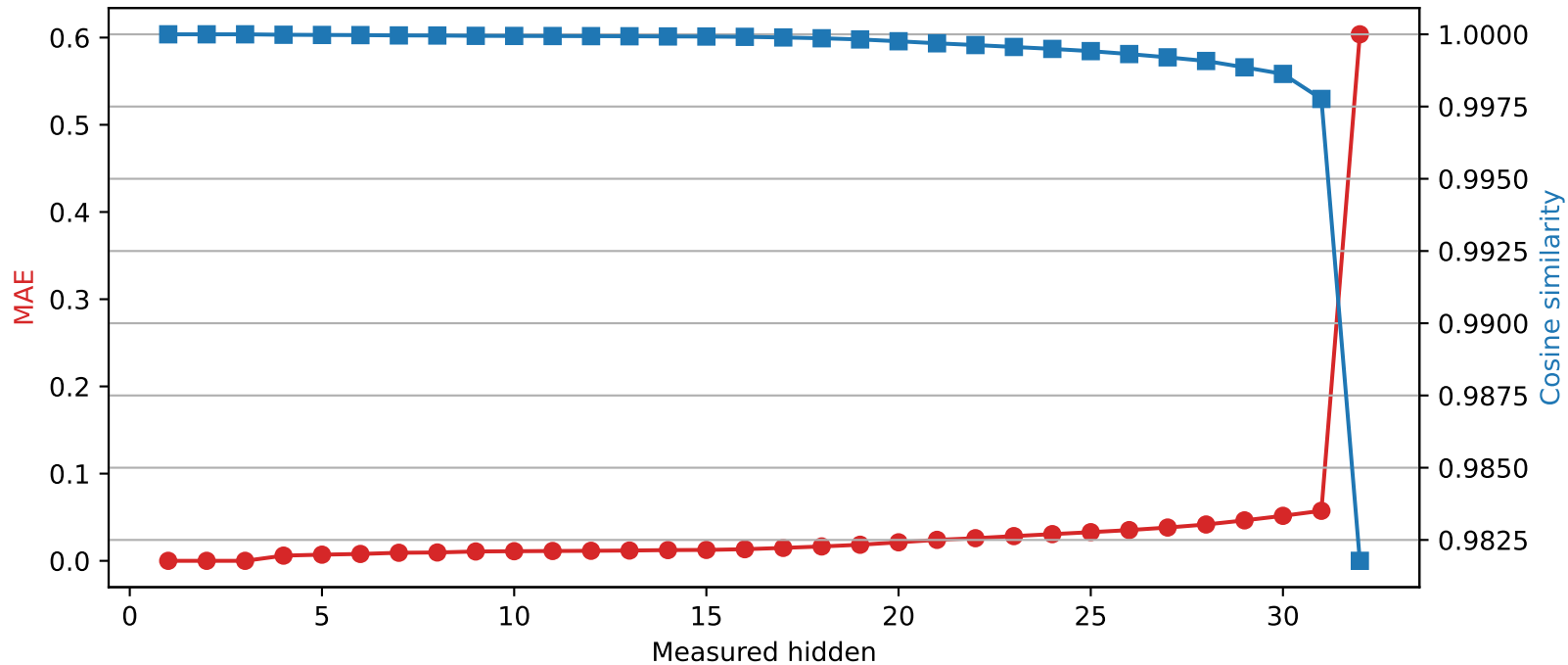
Mistral-7B-Instruct-v0.3 | Quantized layer 3 | float64 → int4
