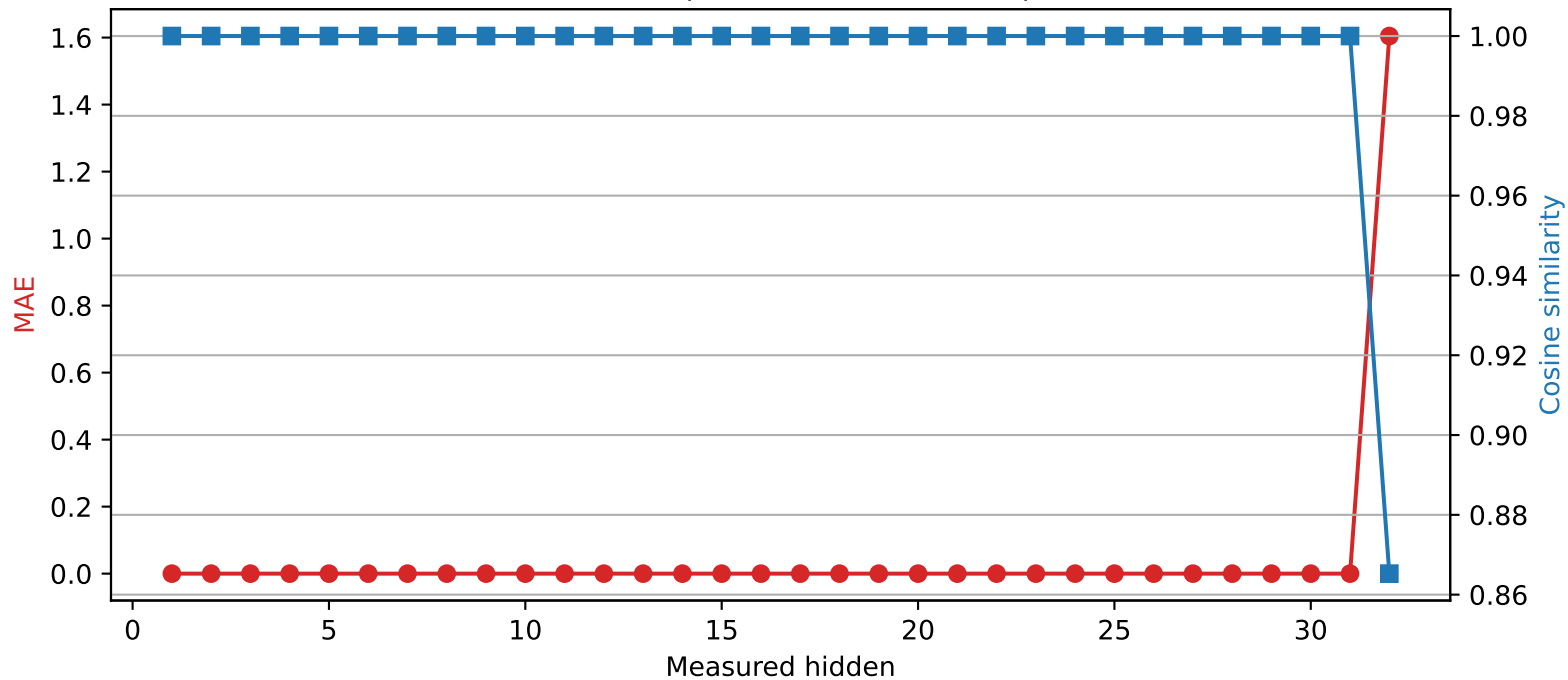
Mistral-7B-Instruct-v0.3 | Quantized layer 31 | float64 \rightarrow int4
