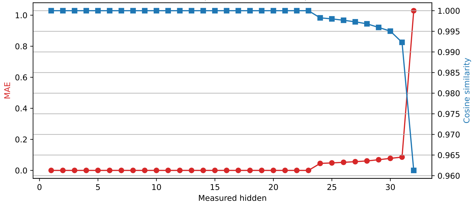
Mistral-7B-Instruct-v0.3 | Quantized layer 23 | float64 → int4
