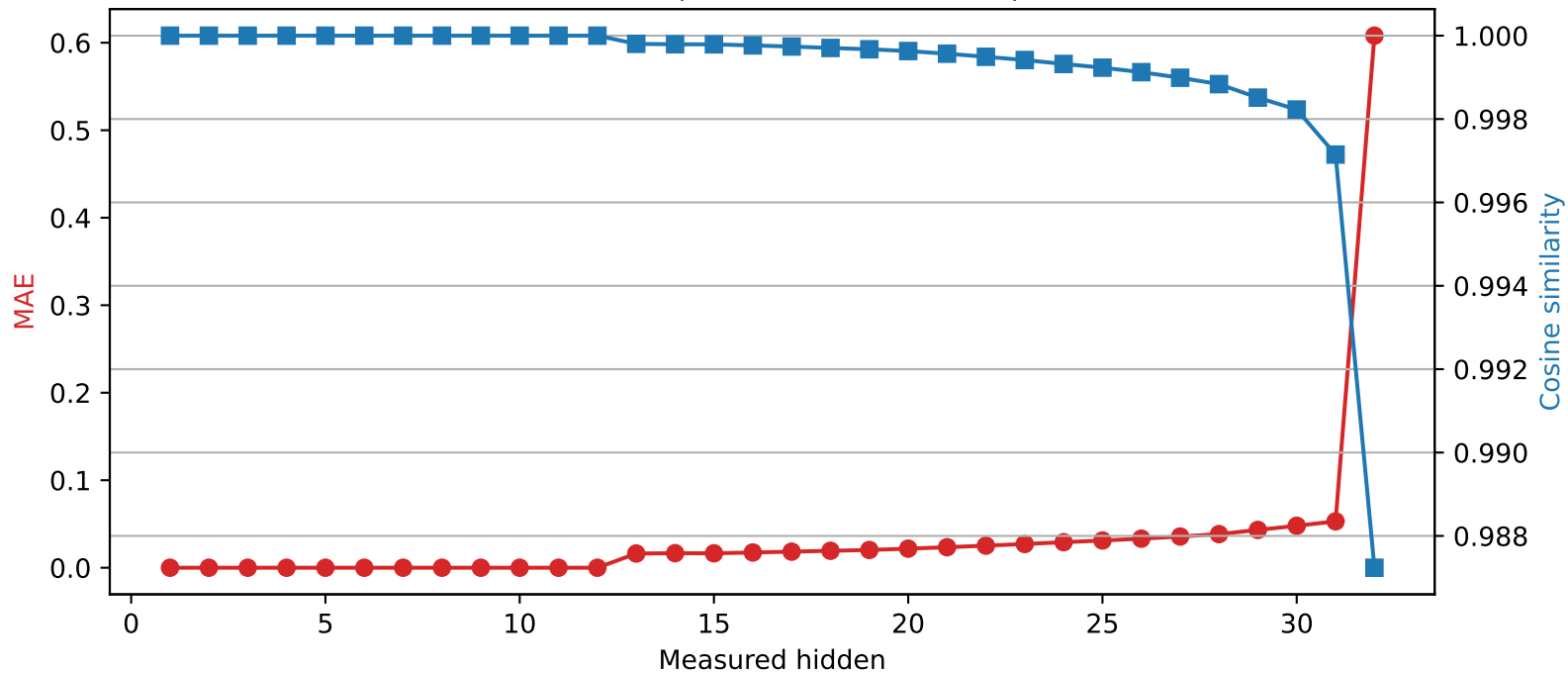
Mistral-7B-Instruct-v0.3 | Quantized layer 12 | float64 → int4
