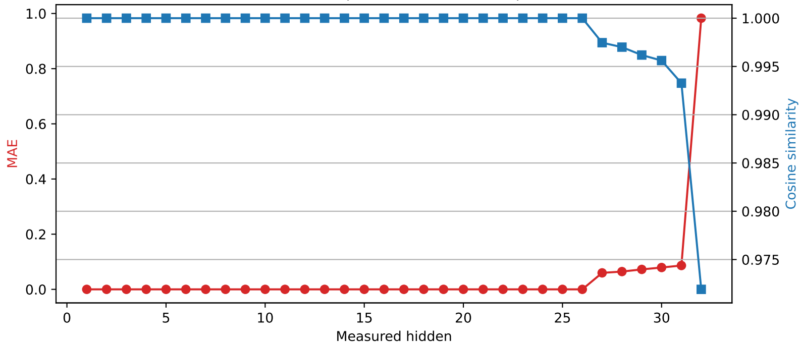
Mistral-7B-Instruct-v0.3 | Quantized layer 26 | float64 → int4
