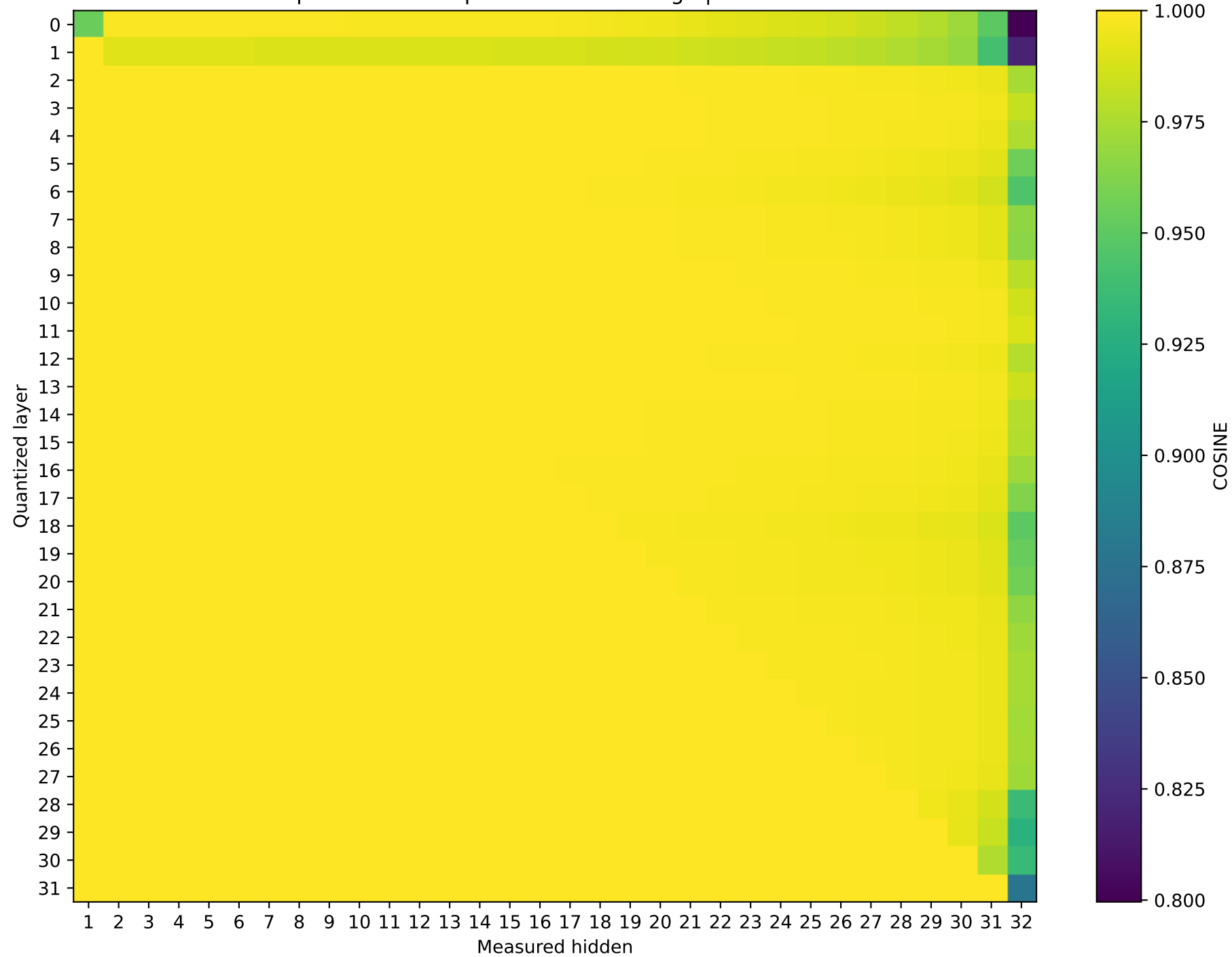
Mistral-7B-Instruct-v0.3 Prompt 3: cos sim representation damage | float64 → int4
