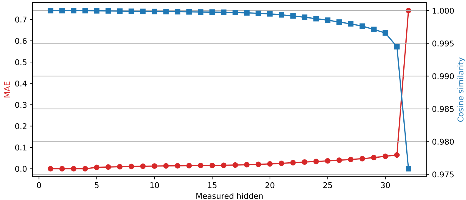
Mistral-7B-Instruct-v0.3 | Quantized layer 4 | float64 → int4
