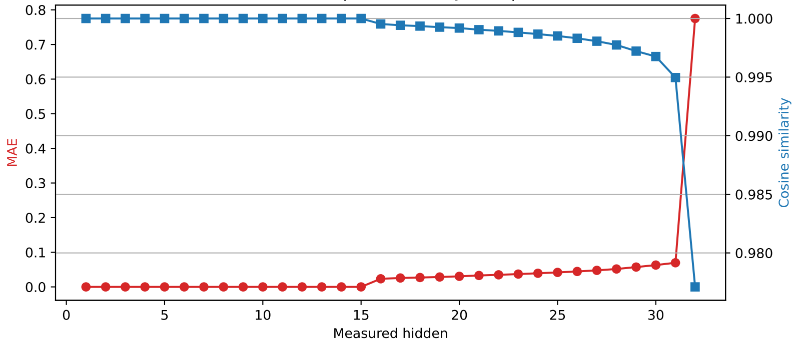
Mistral-7B-Instruct-v0.3 | Quantized layer 15 | float64 → int4
