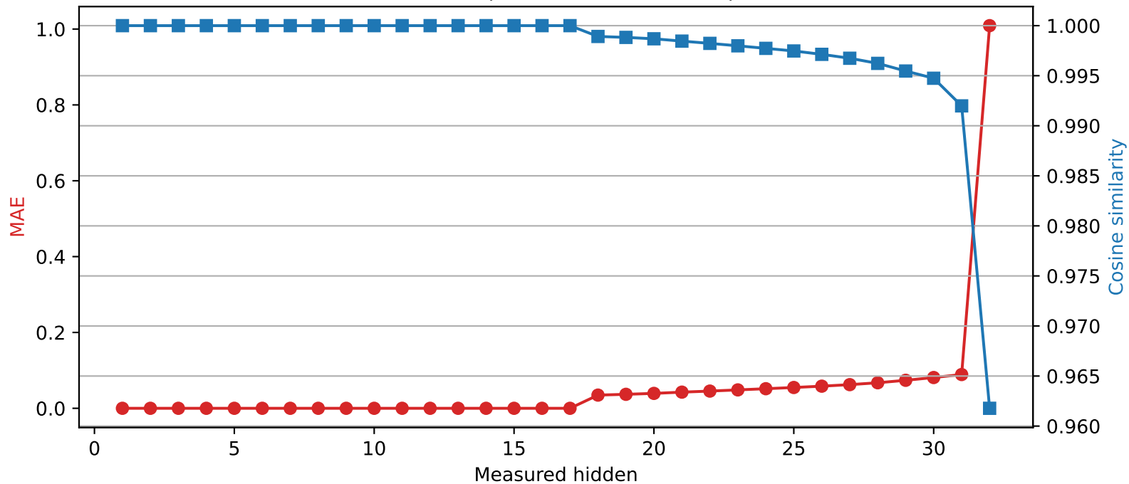
Mistral-7B-Instruct-v0.3 | Quantized layer 17 | float64 → int4
