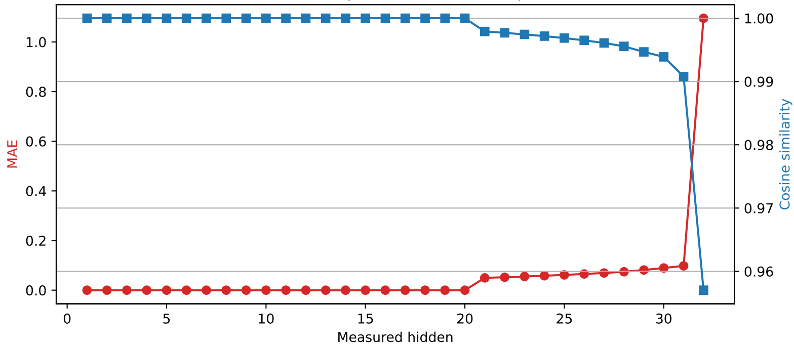
Mistral-7B-Instruct-v0.3 | Quantized layer 20 | float64 → int4
