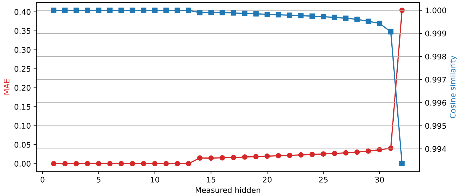
Mistral-7B-Instruct-v0.3 | Quantized layer 13 | float16 \rightarrow int2
