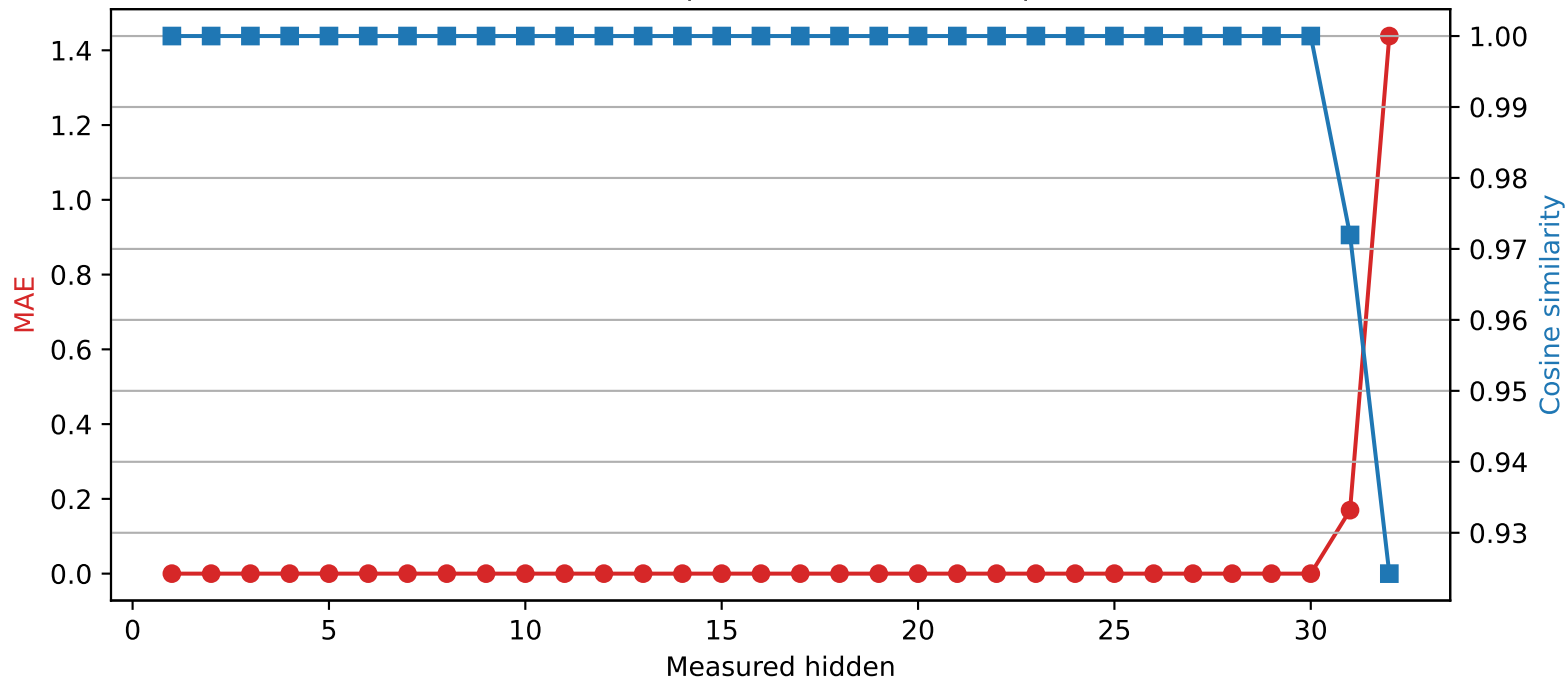
Mistral-7B-Instruct-v0.3 | Quantized layer 30 | float16 → int2
