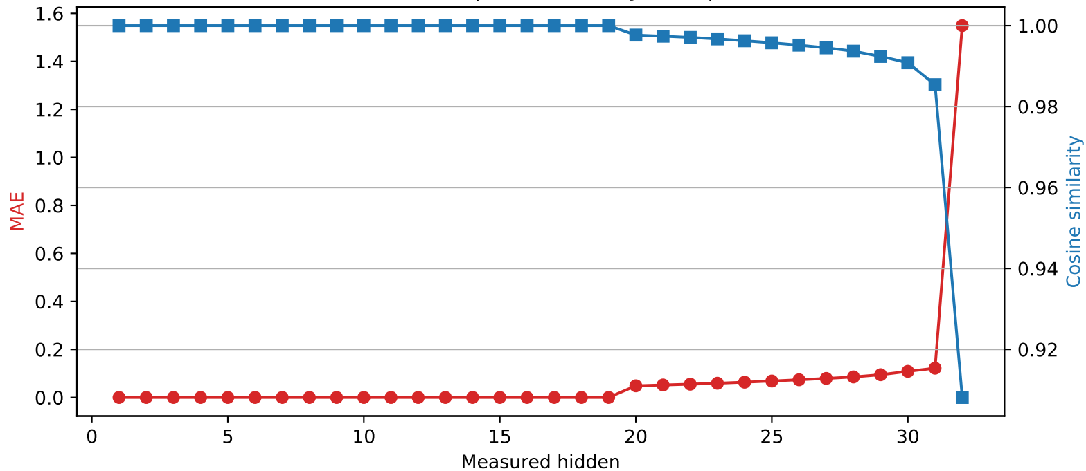
Mistral-7B-Instruct-v0.3 | Quantized layer 19 | float16 → int2
