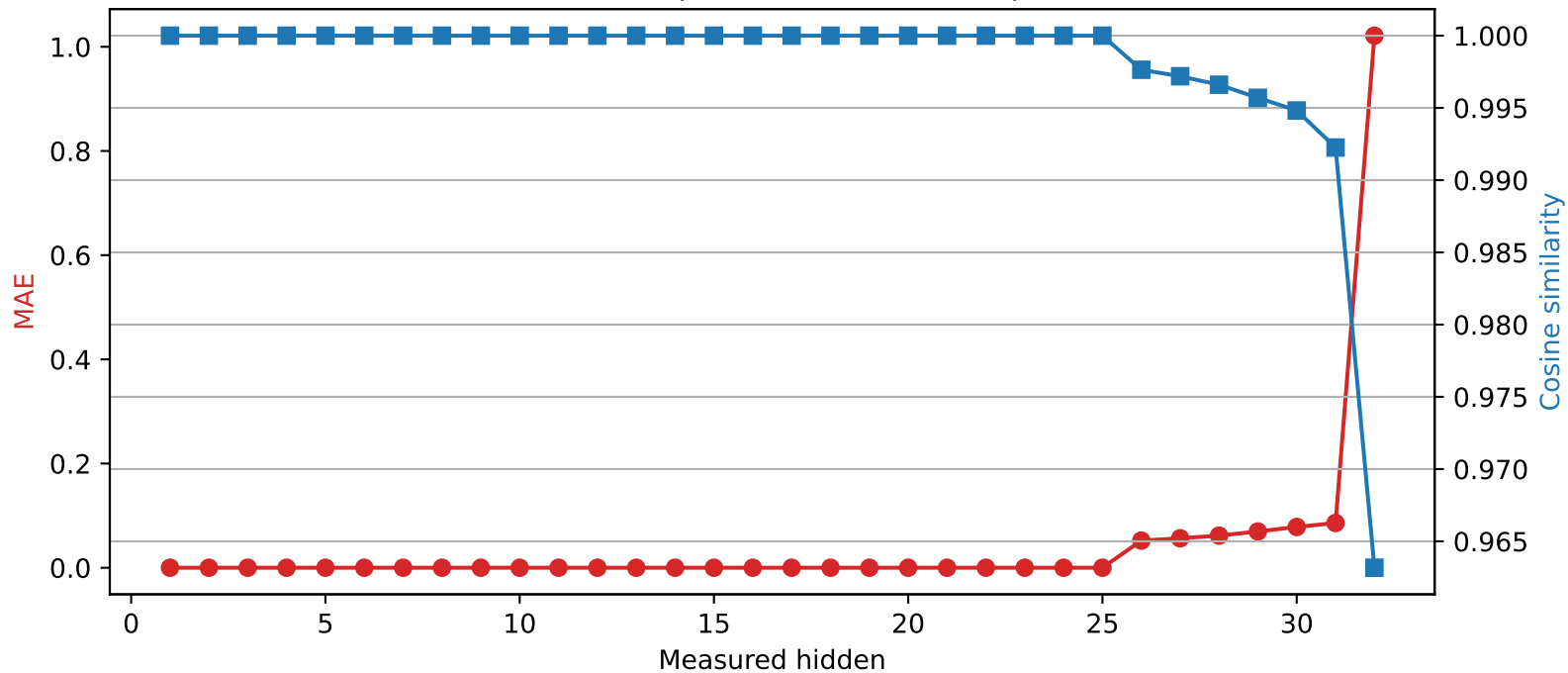
Mistral-7B-Instruct-v0.3 | Quantized layer 25 | float16 → int2
