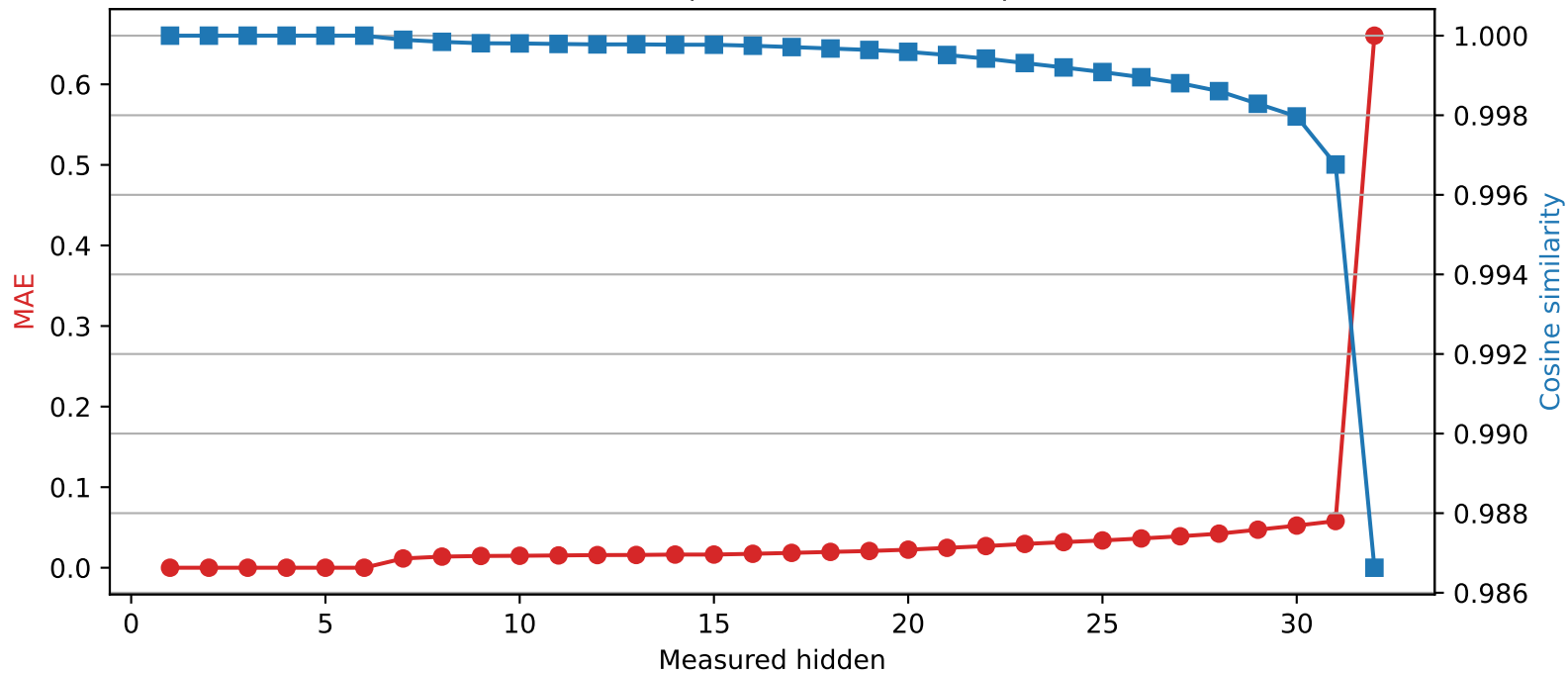
Mistral-7B-Instruct-v0.3 | Quantized layer 6 | float16 \rightarrow int2
