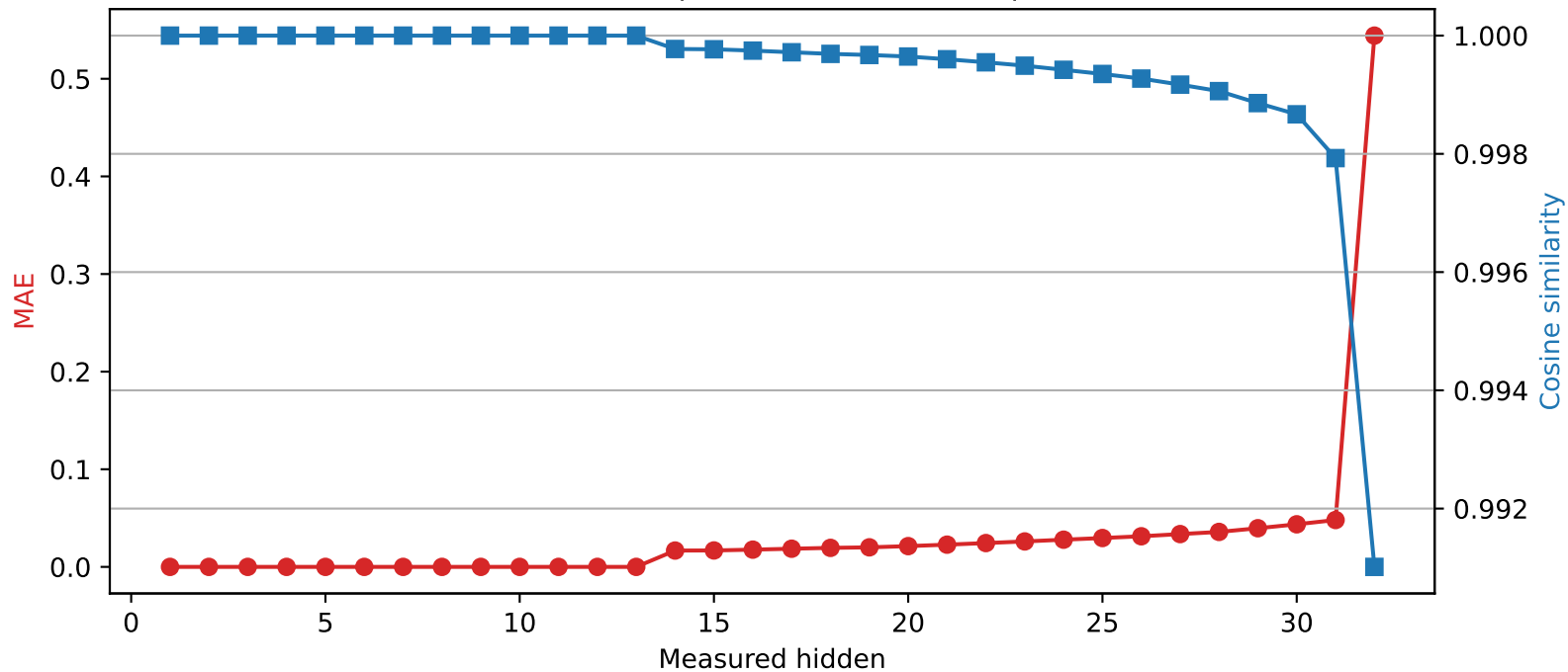
Mistral-7B-Instruct-v0.3 | Quantized layer 13 | float16 → int2
