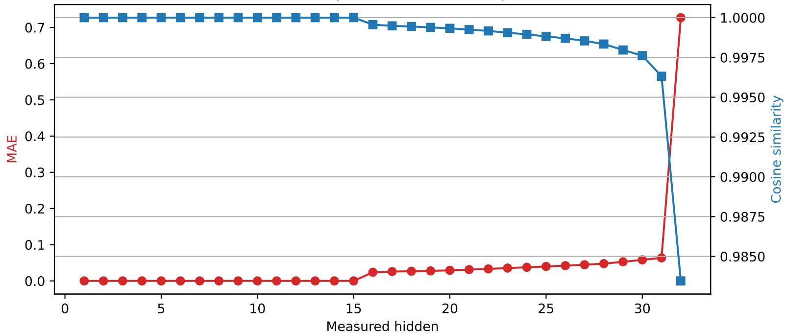
Mistral-7B-Instruct-v0.3 | Quantized layer 15 | float16 → int2
