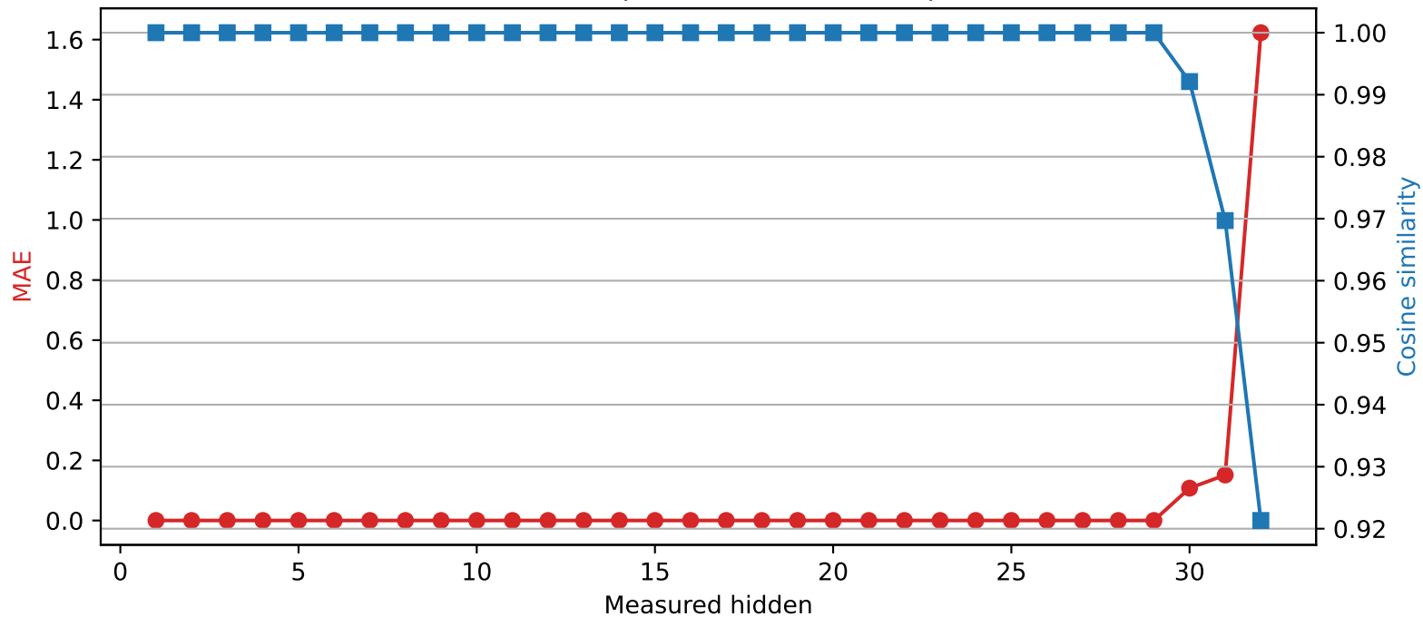
Mistral-7B-Instruct-v0.3 | Quantized layer 29 | float16 → int2
