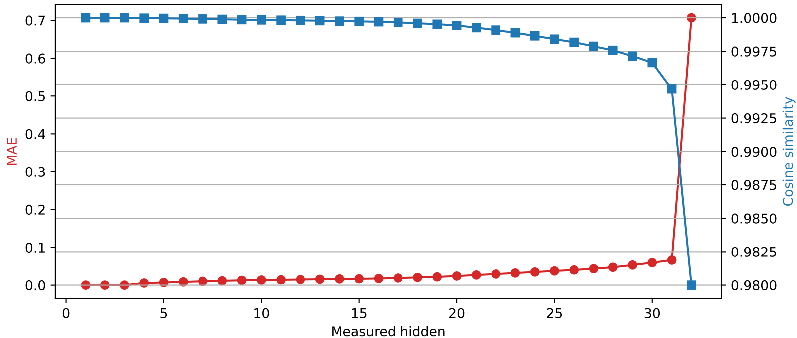
Mistral-7B-Instruct-v0.3 | Quantized layer 3 | float16 → int2
