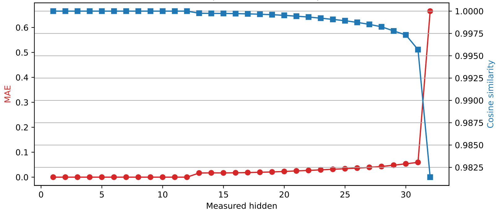
Mistral-7B-Instruct-v0.3 | Quantized layer 12 | float16 → int2
