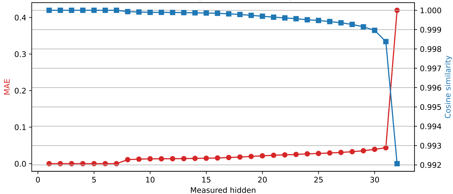
Mistral-7B-Instruct-v0.3 | Quantized layer 7 | float16 → int2
