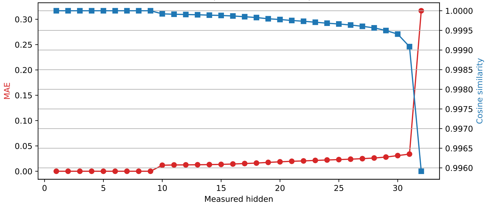
Mistral-7B-Instruct-v0.3 | Quantized layer 9 | float16 → int2
