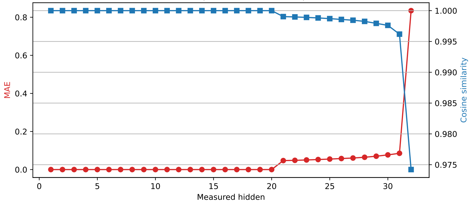
Mistral-7B-Instruct-v0.3 | Quantized layer 20 | float32 \rightarrow int2
