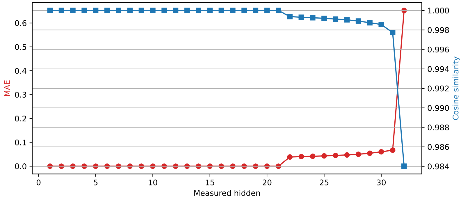
Mistral-7B-Instruct-v0.3 | Quantized layer 21 | float32 → int2
