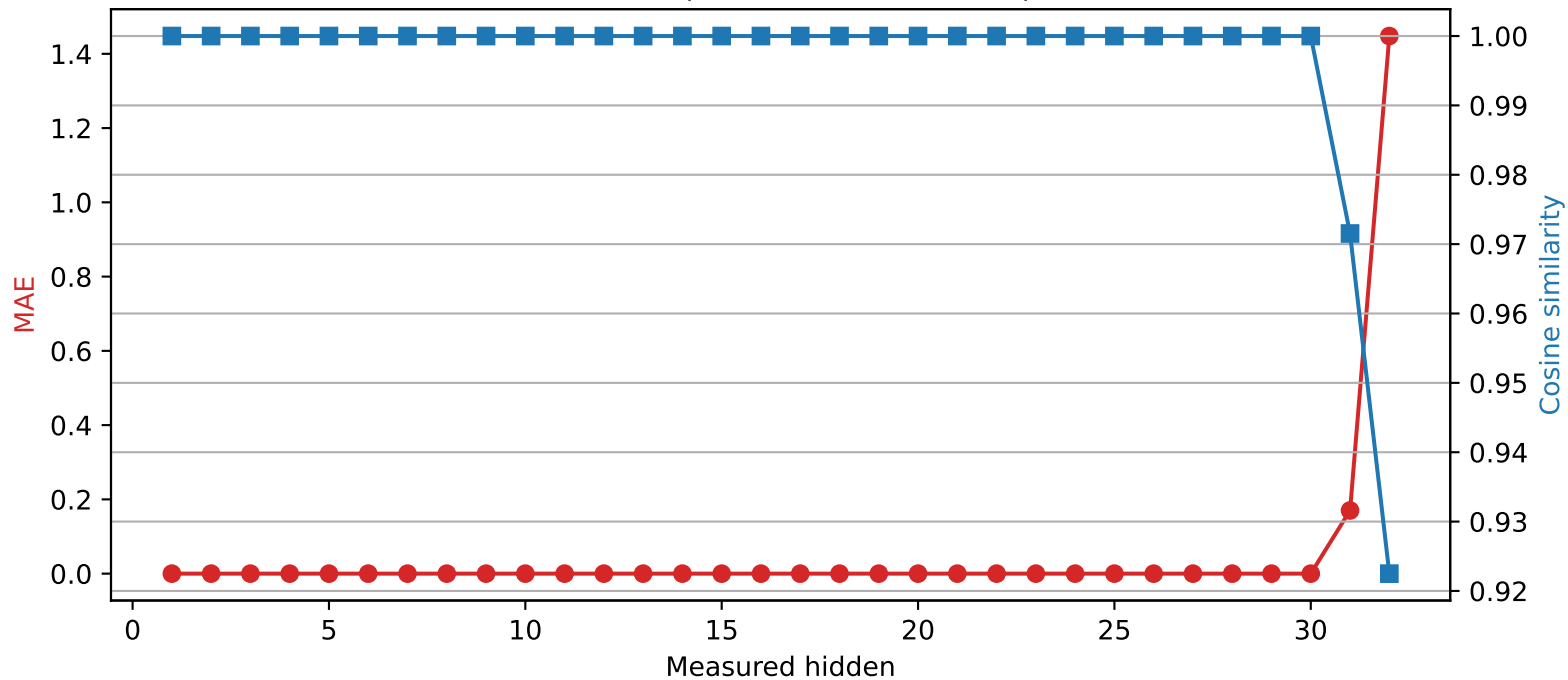
Mistral-7B-Instruct-v0.3 | Quantized layer 30 | float32 → int2
