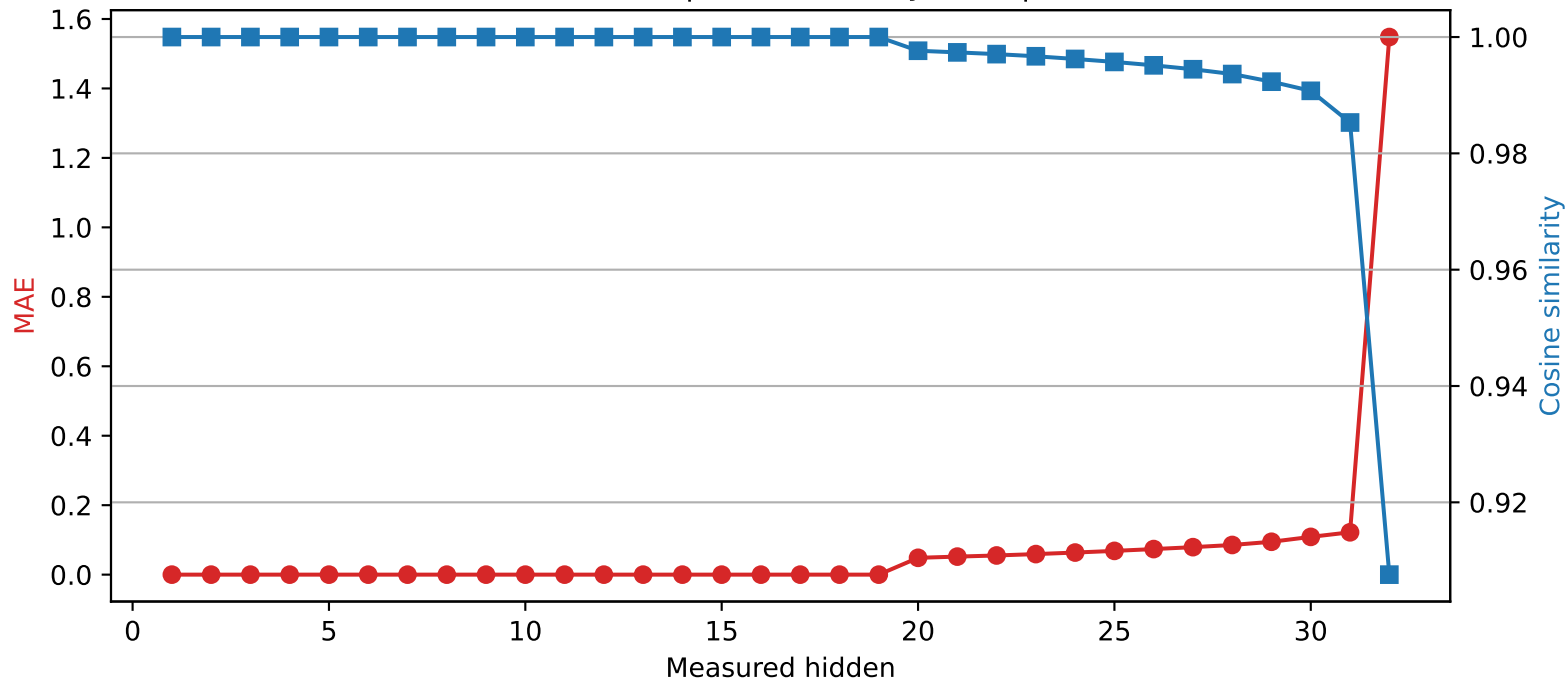
Mistral-7B-Instruct-v0.3 | Quantized layer 19 | float32 → int2
