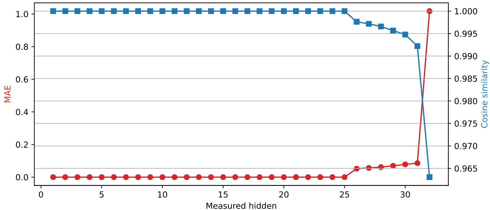
Mistral-7B-Instruct-v0.3 | Quantized layer 25 | float32 → int2
