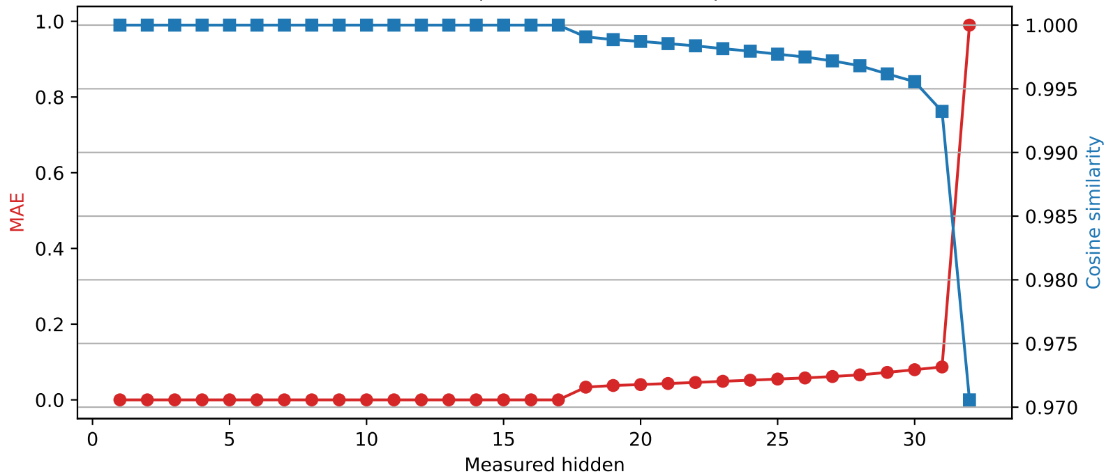
Mistral-7B-Instruct-v0.3 | Quantized layer 17 | float32 → int2
