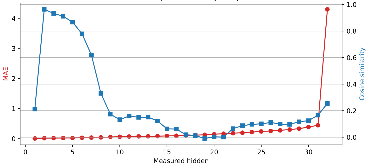
Mistral-7B-Instruct-v0.3 | Quantized layer 0 | float32 → int2
